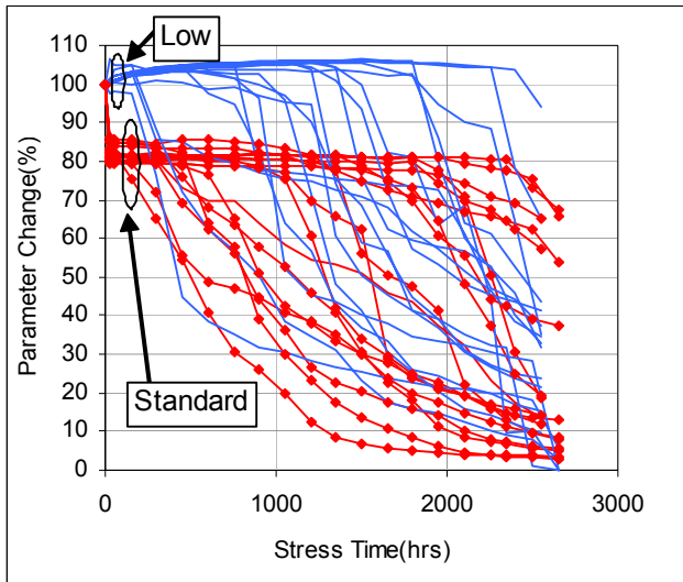
Fig. 5: Normalized Beta degradation for typical InGaP/InGaAsN transistors for both standard and low burn-in material.
