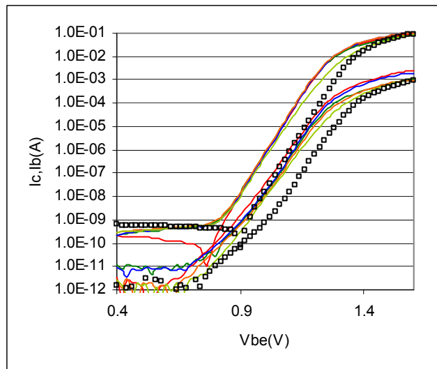
Fig 1. Gummel plots for InGaP/GaAs HBT's, shown in squares, and InGaP/InGaAsN variants shown in lines.
