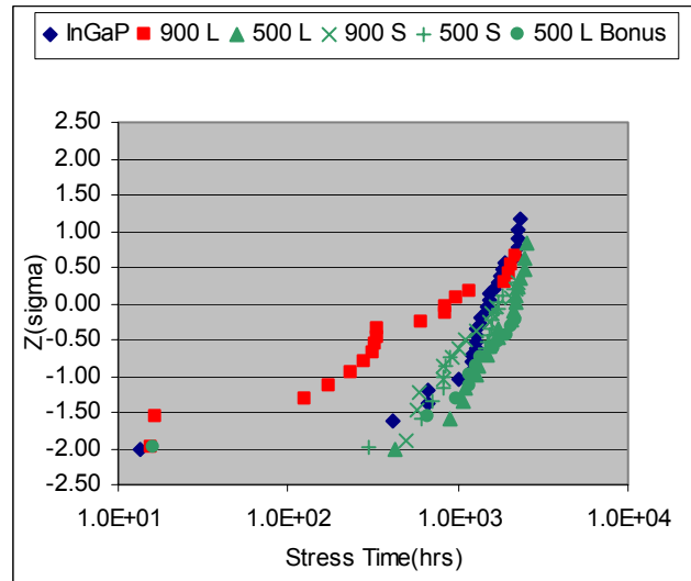
Fig. 6: Cumulative failures transformed into linear space for control and InGaP/InGaAsN variants. Z=0 is equivalent to MTTF. The number in the legend indicates the base thickness and the letters S and L denote standard or low burn-in material.
