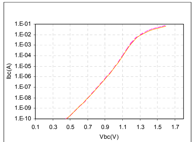
Fig. 4: Typical forward BC diode for InGaP/InGaAsN transistor showing stable I_c for length of stress test.
