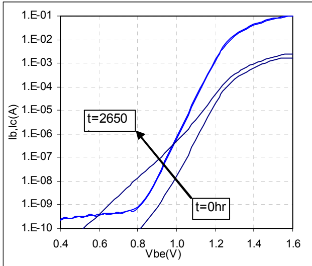
Fig. 2: Gummel plot for Typical InGaP/InGaAsN showing fundamental failure mode as Beta degradation due to degradation in I_b .
