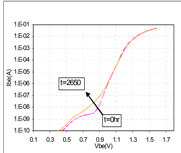
Fig. 3: Typical forward BE diode for InGaP/InGaAsN transistor showing degradation in I_b .
